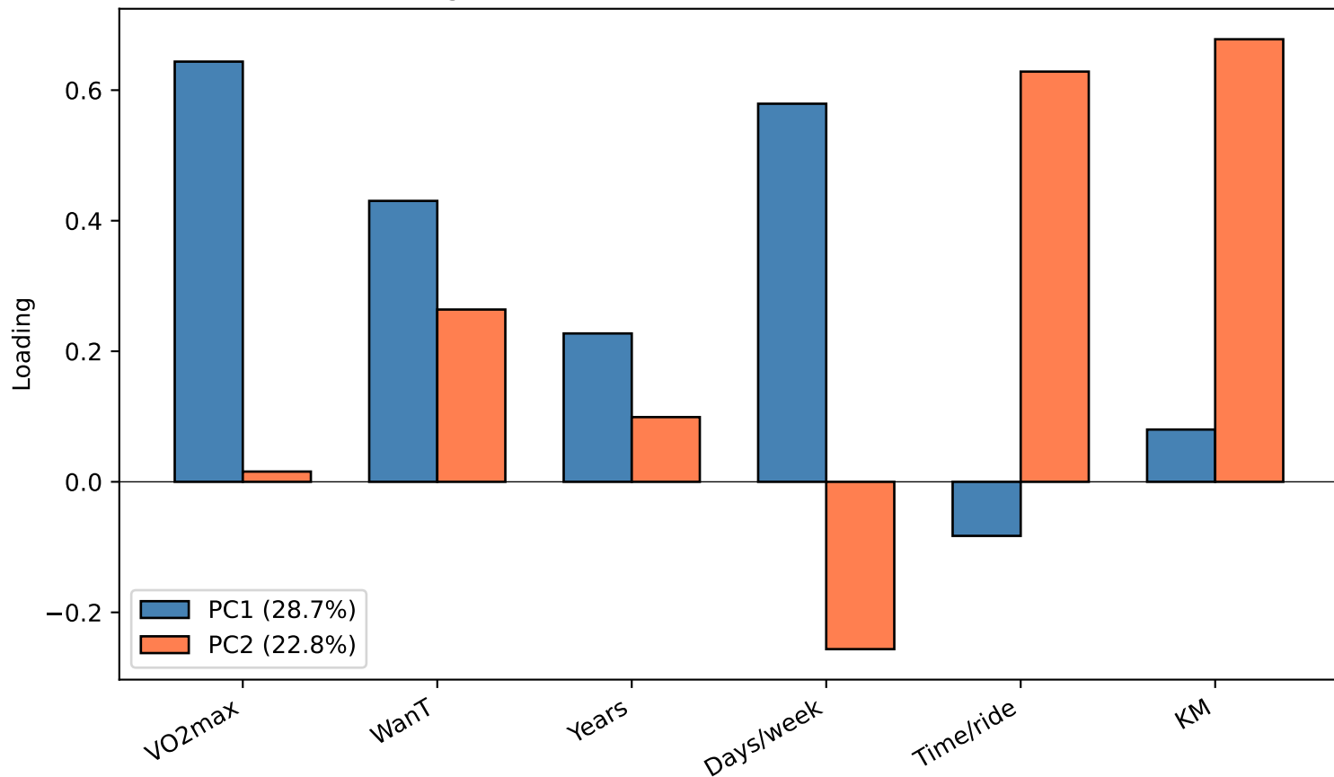
PCA Loadings — Contribution of Each Variable to PC1 and PC2
