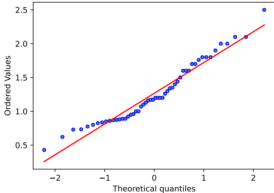
Q-Q Plot
