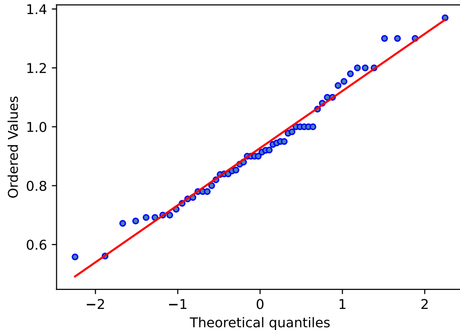
Q-Q Plot
