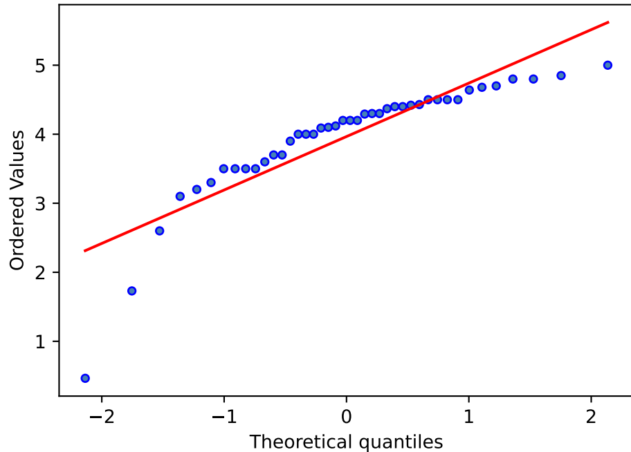
Q-Q Plot
