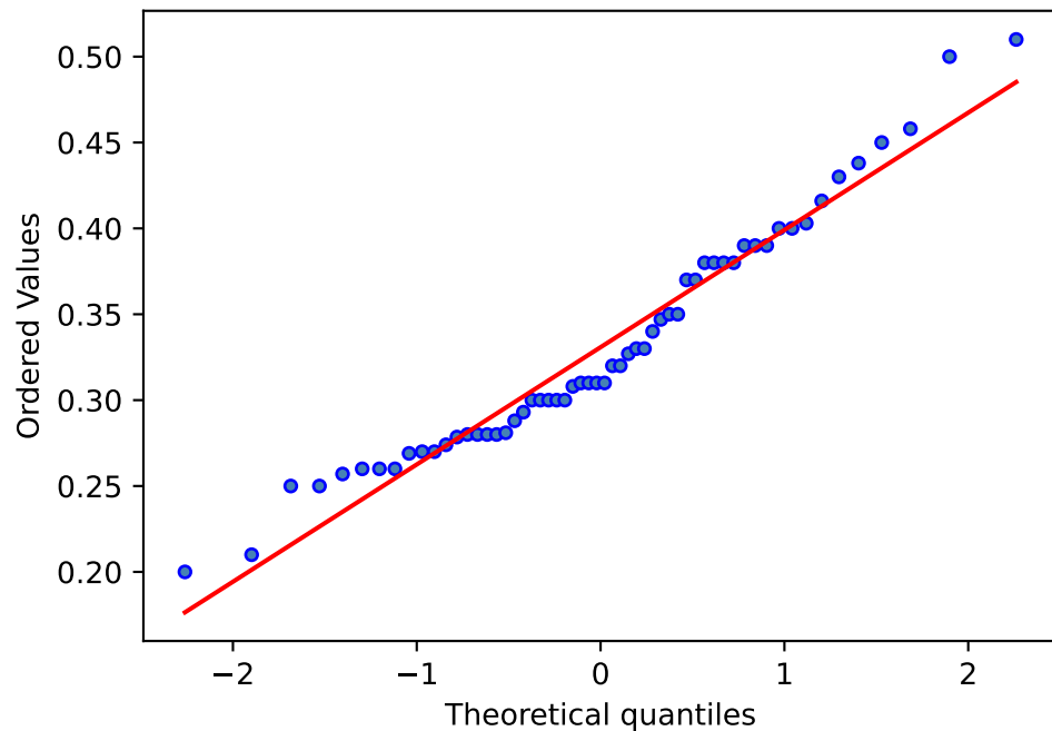
Q-Q Plot
