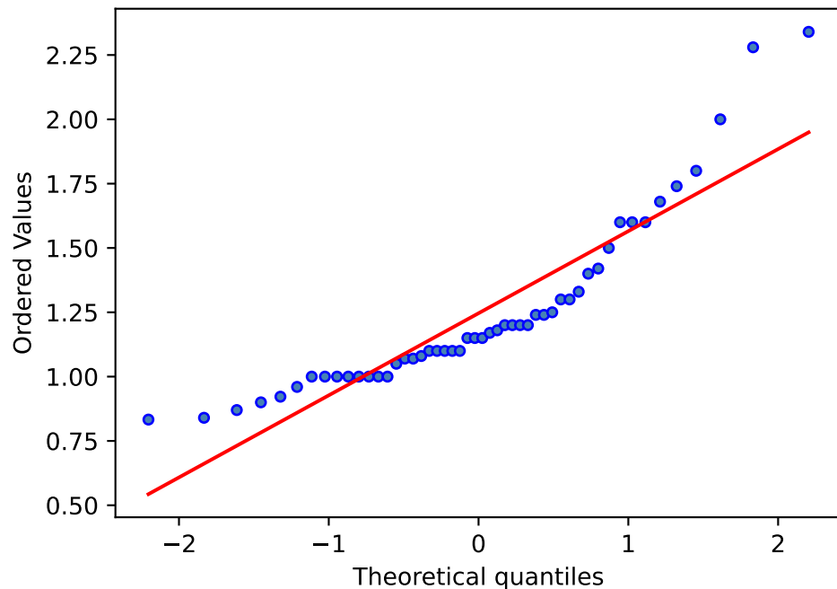
Q-Q Plot
