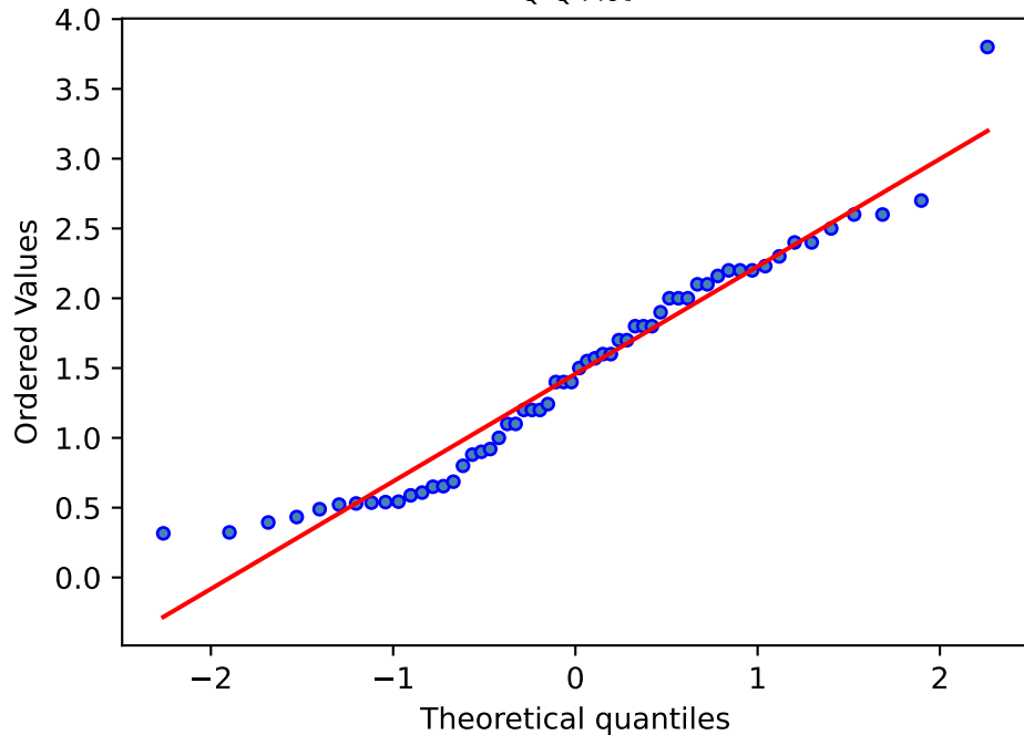
Q-Q Plot
