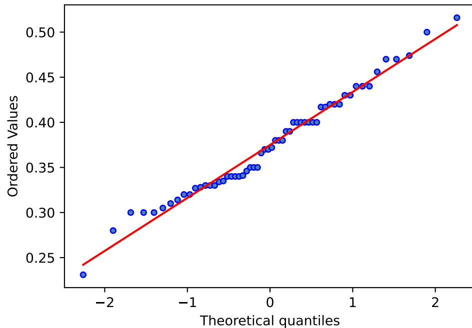
Q-Q Plot
