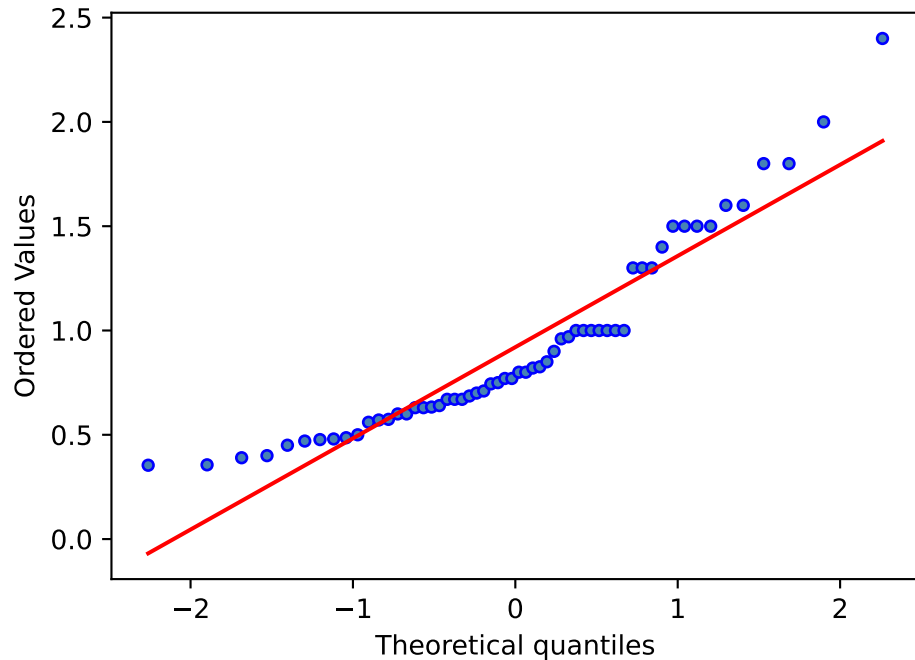
Q-Q Plot
