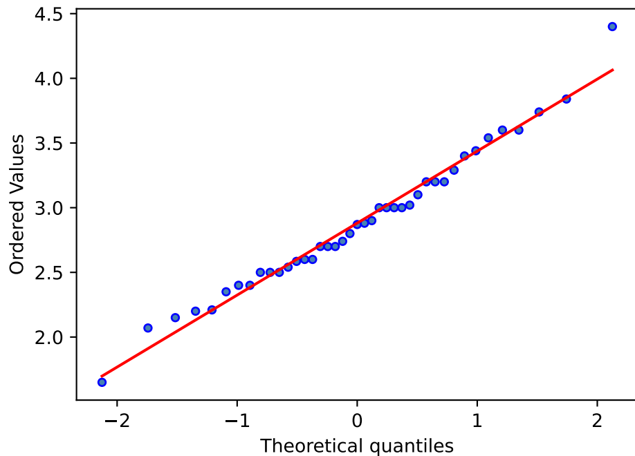
Q-Q Plot
