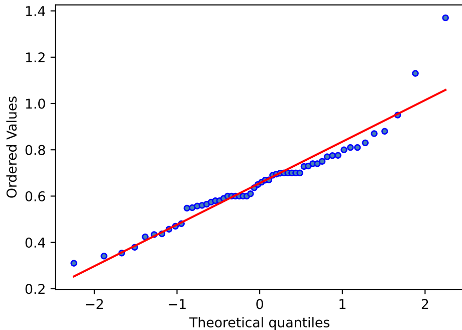
Q-Q Plot
