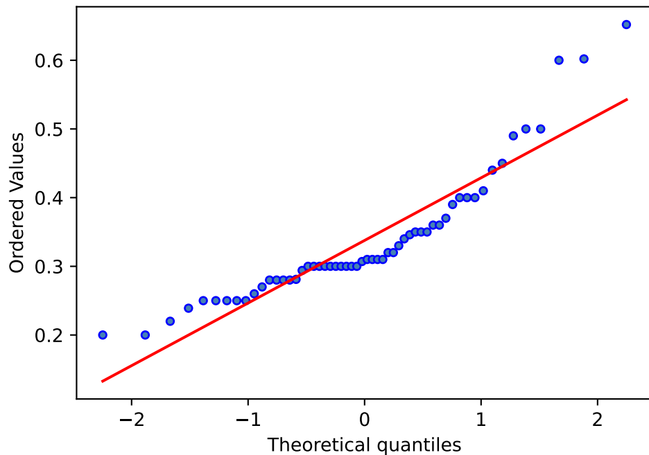
Q-Q Plot
