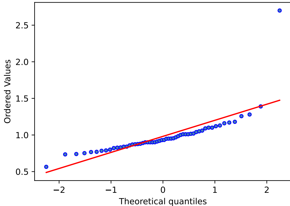
Q-Q Plot
