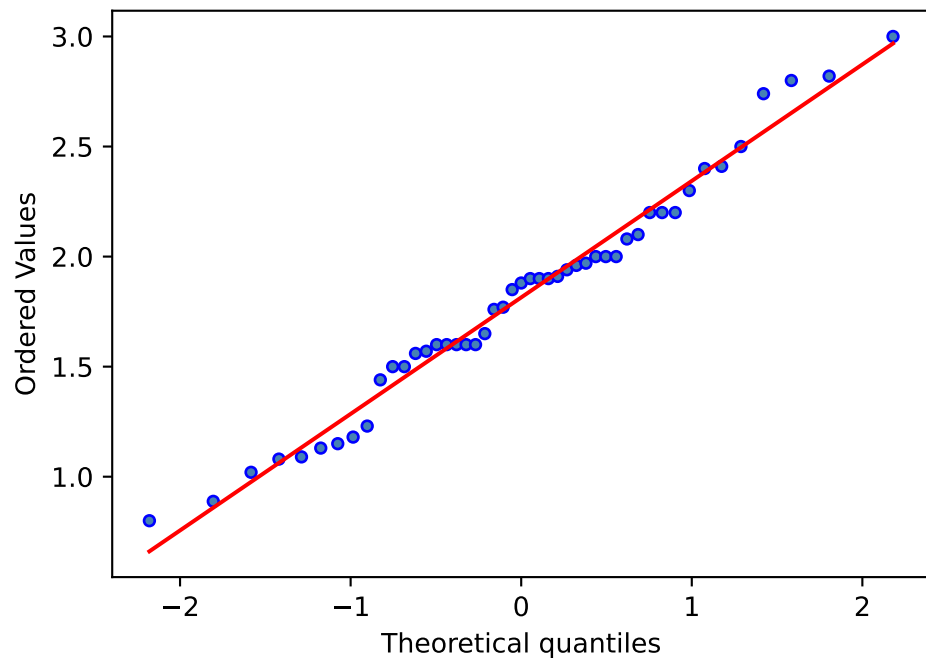
Q-Q Plot
