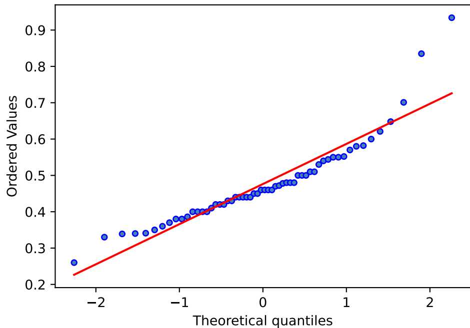
Q-Q Plot
