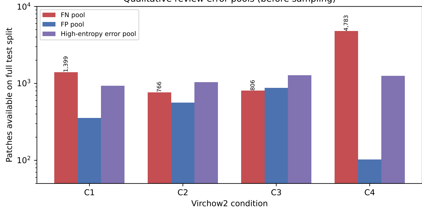
Qualitative review error pools (before sampling)
