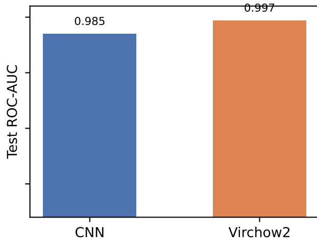
Train PCam Test CAMELYON17 (C2)
