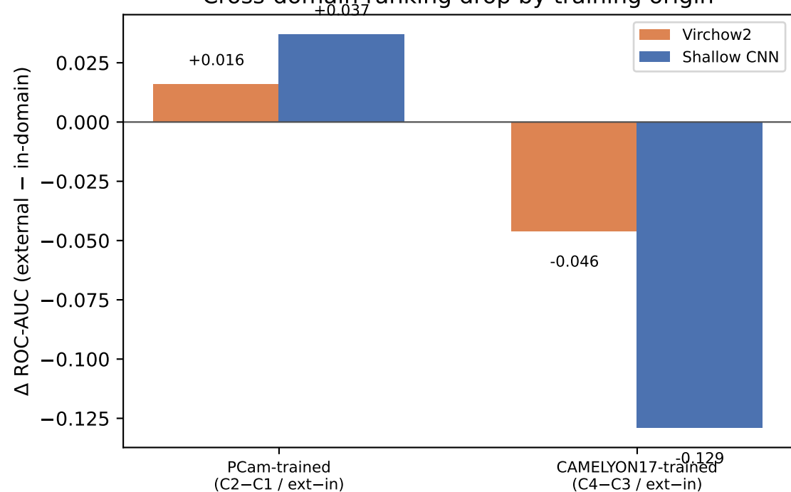
Cross-domain ranking drop by training origin
