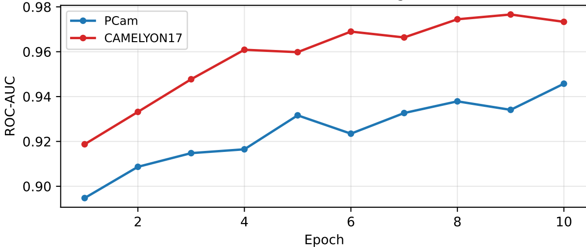
Validation ROC-AUC (raw sigmoid)
