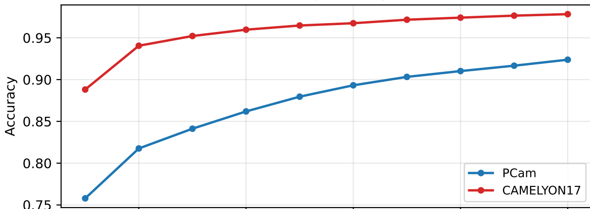
Training accuracy
