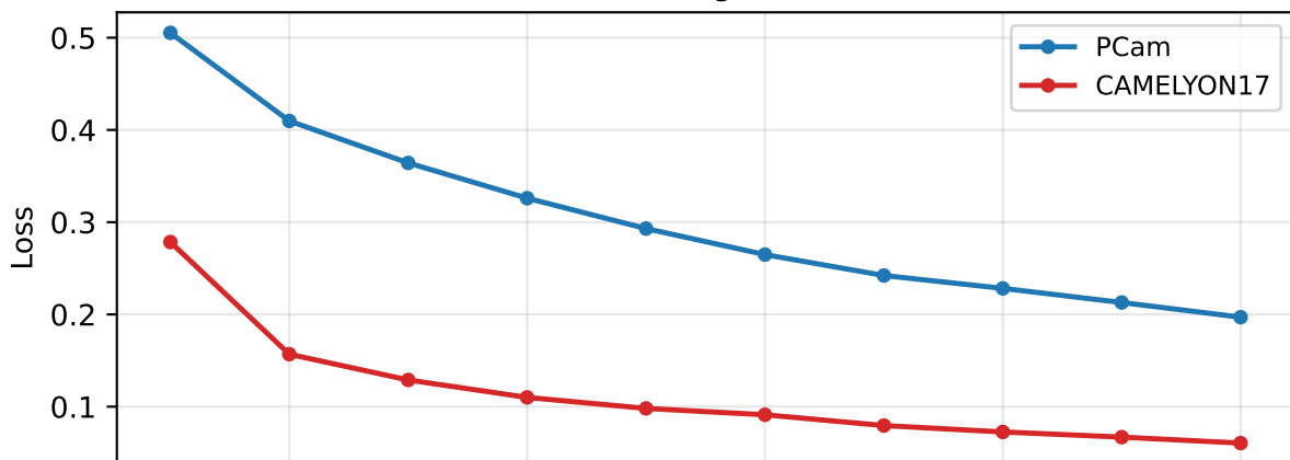
Training loss
