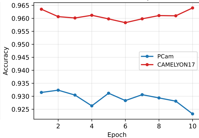
Validation accuracy
