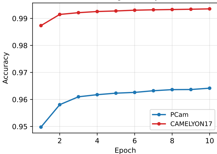
Training accuracy
