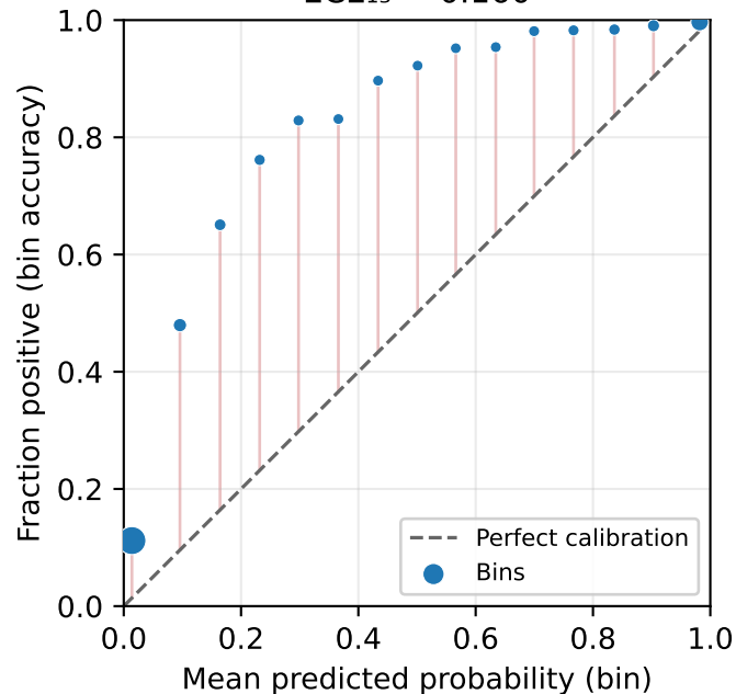
C4: CAMELYON17 \rightarrow PCam test ECE_{15} = 0.160
