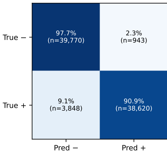
CAMELYON17 → CAMELYON17
