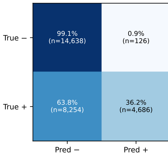
CAMELYON17 → PCam
