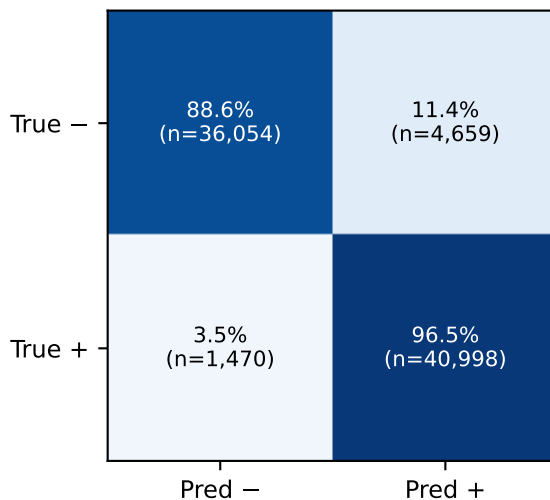
PCam → CAMELYON17
