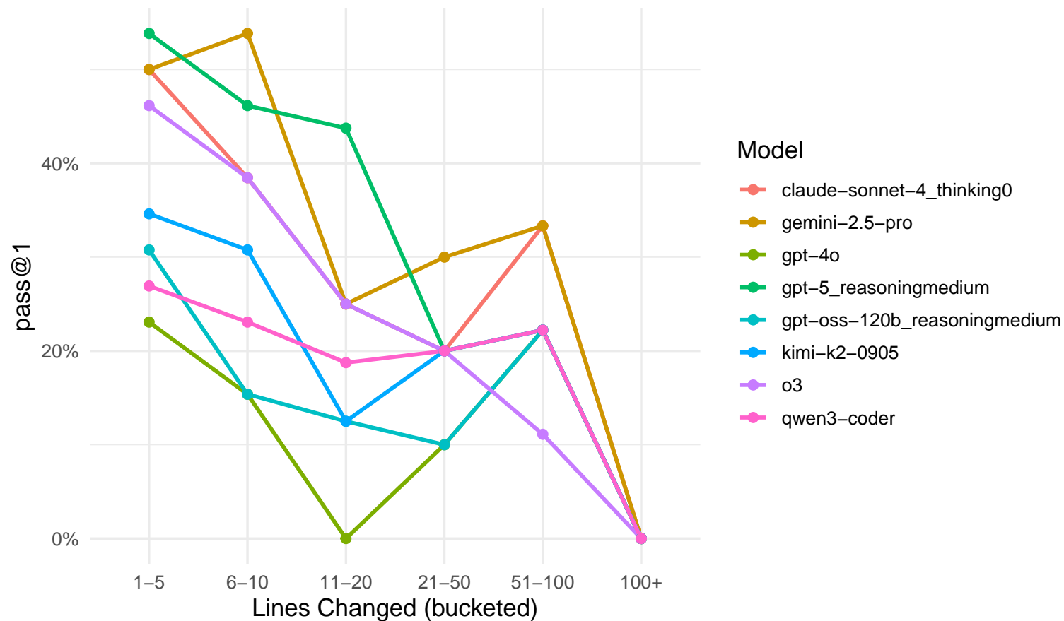
pass@1 vs Lines Changed
