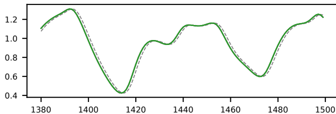
Mackey-Glass: lowest-RMSE RNN = MRN (last 120 of 300 test pts)
