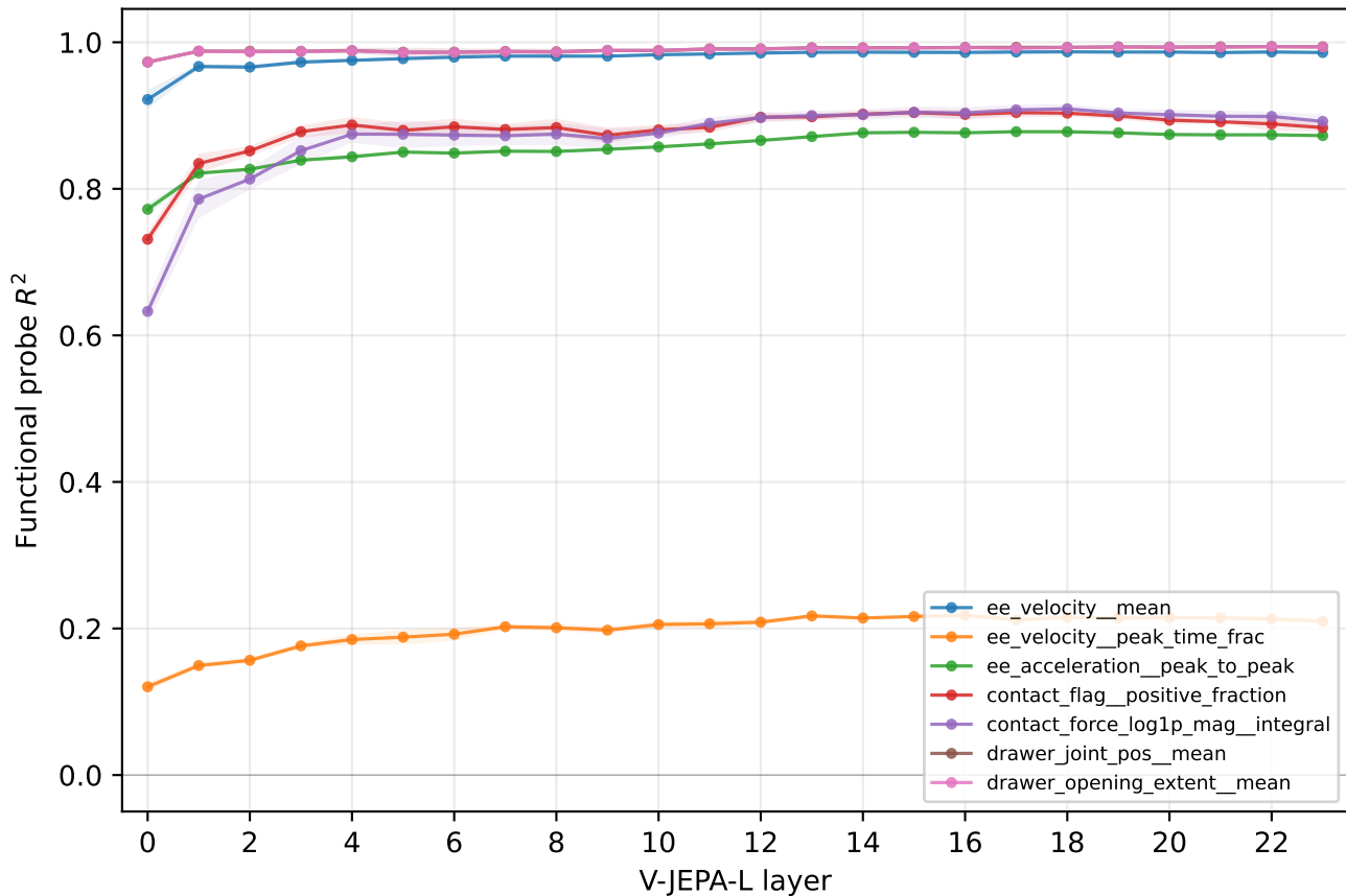
drawer — Variant A functional probe per-target R^2 across 24 layers
