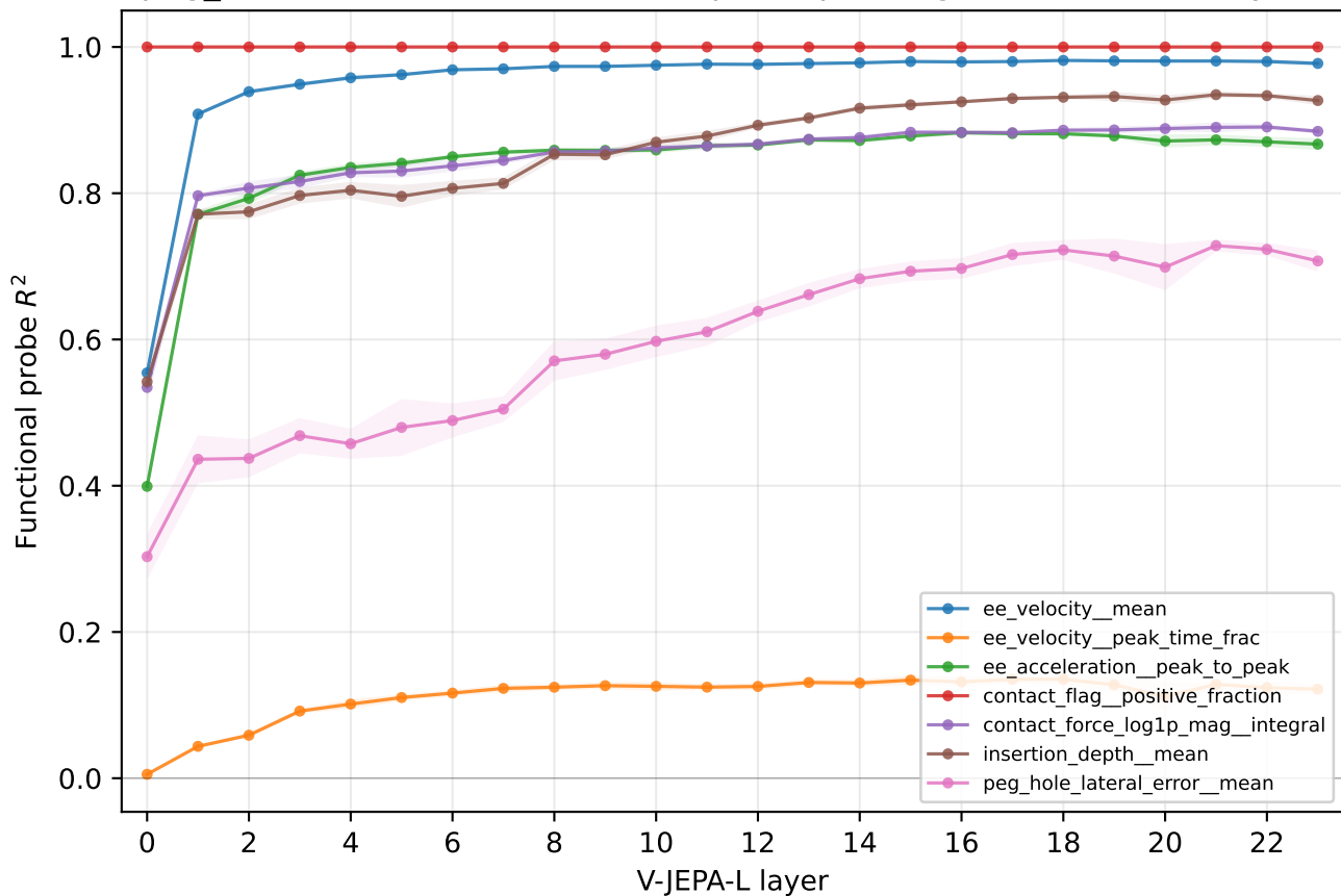
peg_insert — Variant A functional probe per-target R^2 across 24 layers
