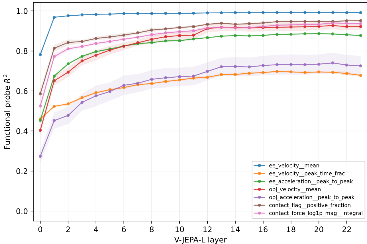
strike — Variant A functional probe per-target R^2 across 24 layers
