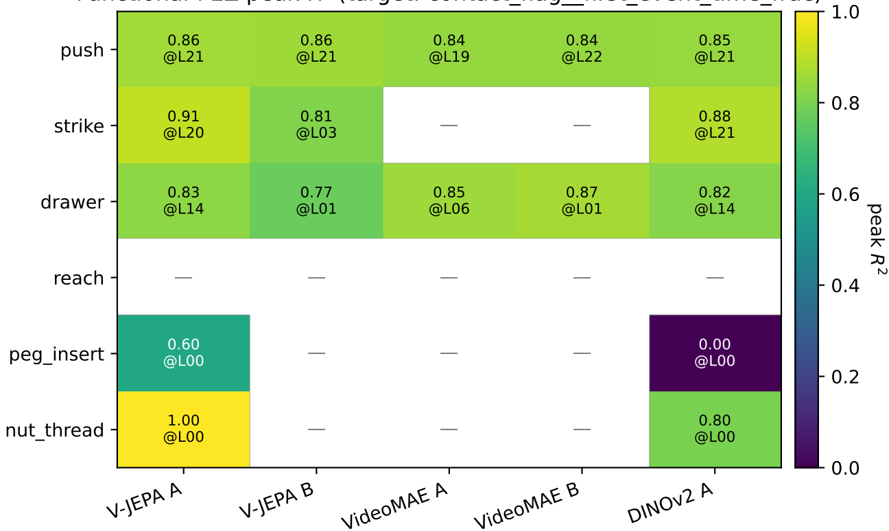
Functional-PEZ peak R^2 (target: contact_flag__first_event_time_frac)
