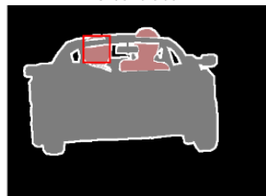
Ground truth
