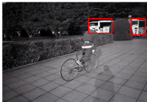
Image
