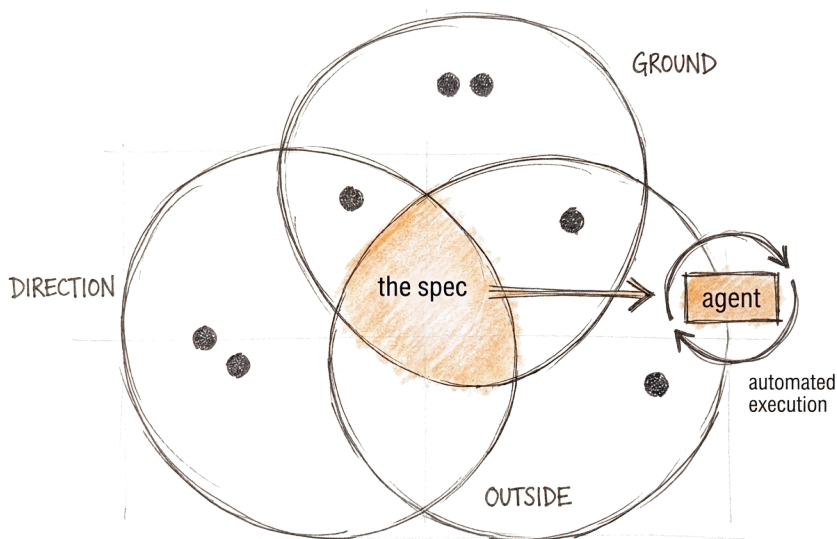
Figure 3: Direction, ground, and outside overlap into the spec; the agent runs only from that overlap.
