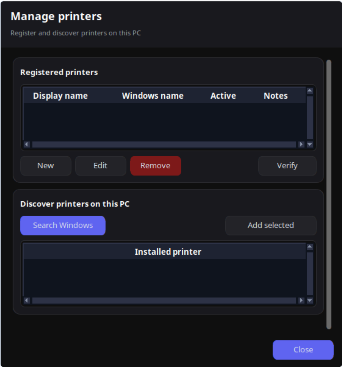
Figure 3 — Register Windows printer names and friendly display names.
