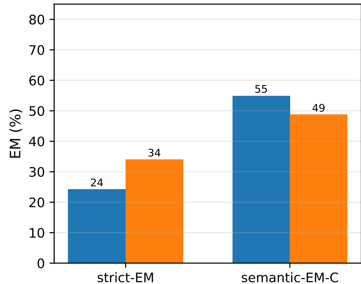
Overall (n=358)
