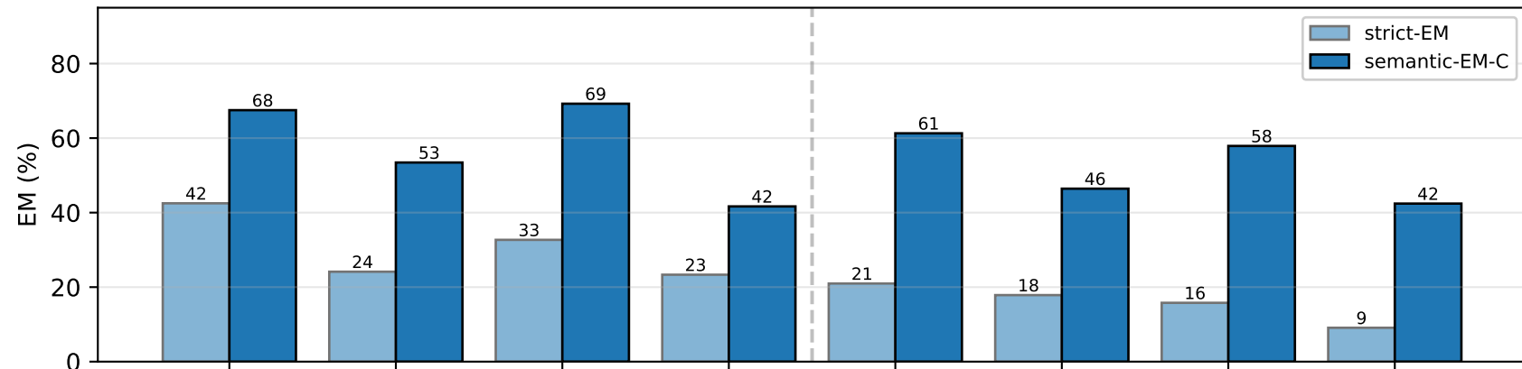
Qwen2.5-VL-7B
