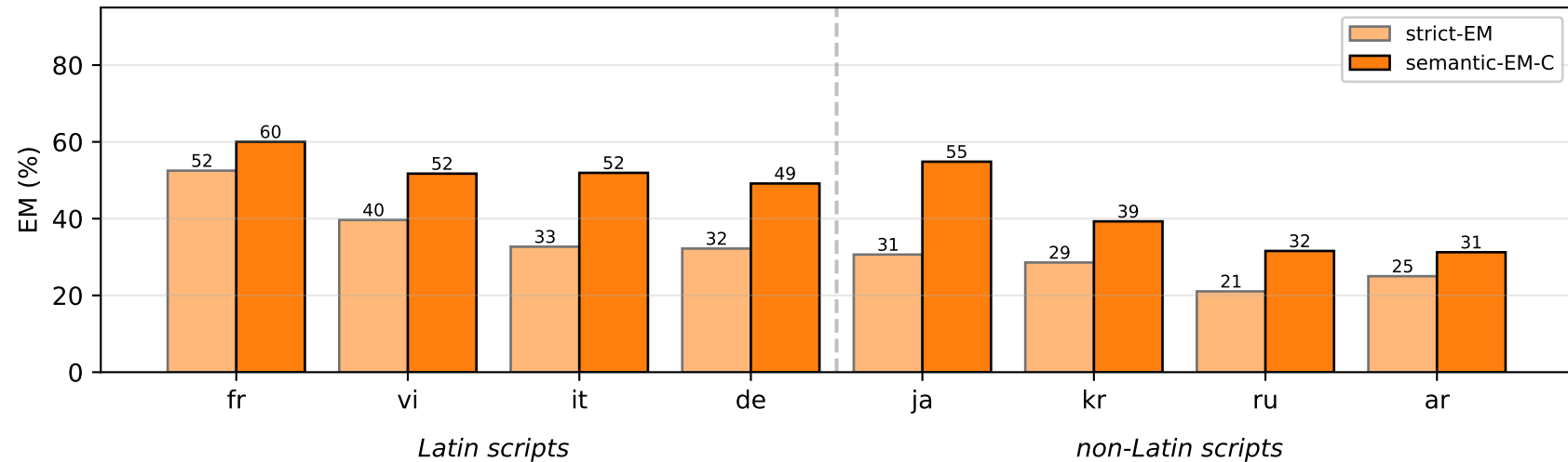
InternVL-2.5-8B
