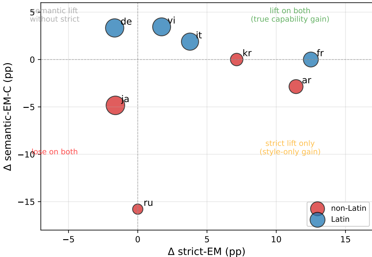
Per-language SFT (d16, 6054 pairs) lift decomposition Qwen2.5-VL-7B base \rightarrow d16, MTVQA 358 held-out
