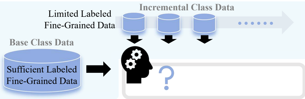
(a) Existing learning paradigms
