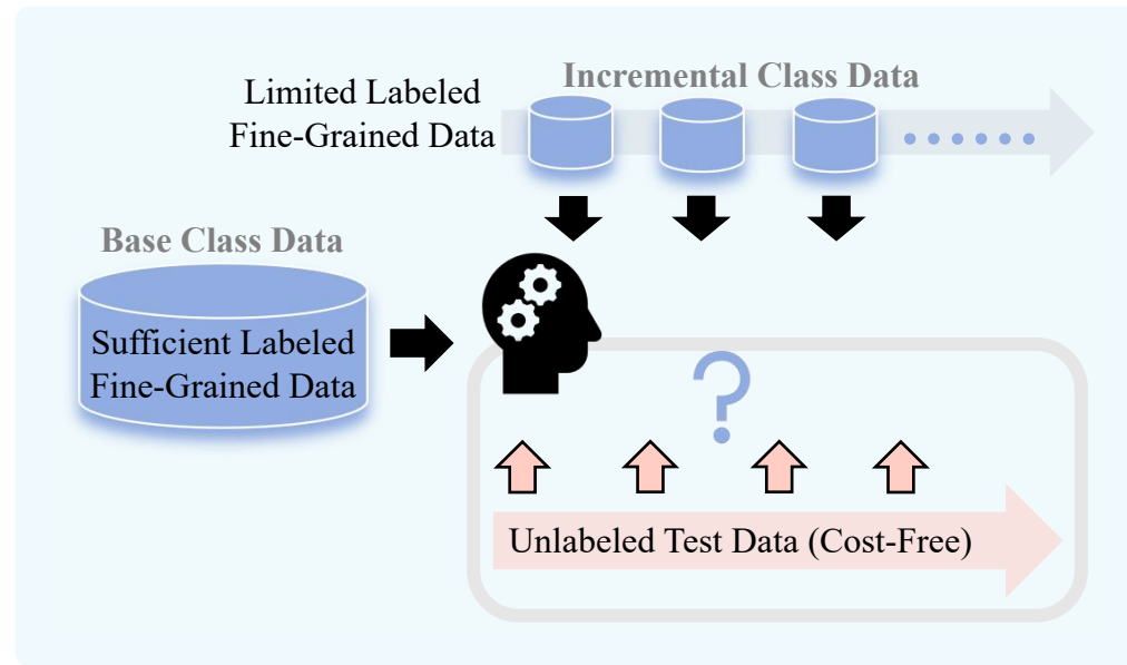
(b) Our learning paradigm
