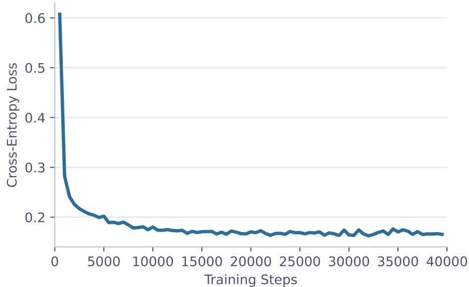
Validation Loss (Run 2)
