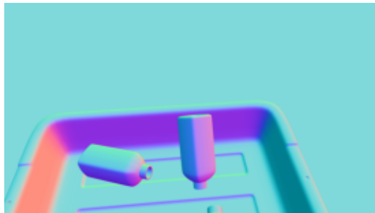
Surface normals
