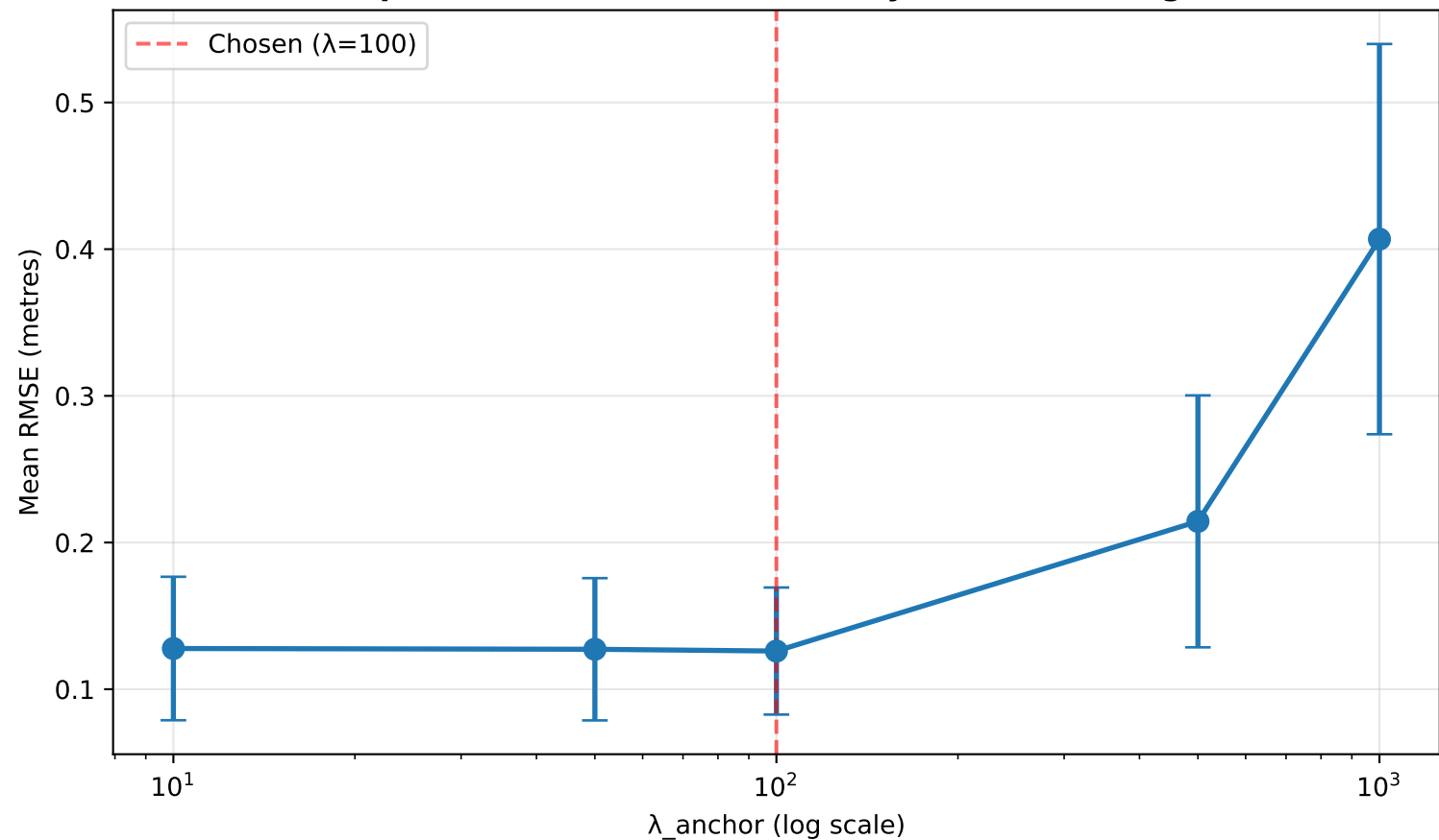
Depth Reconstruction Sensitivity to Anchor Weight
