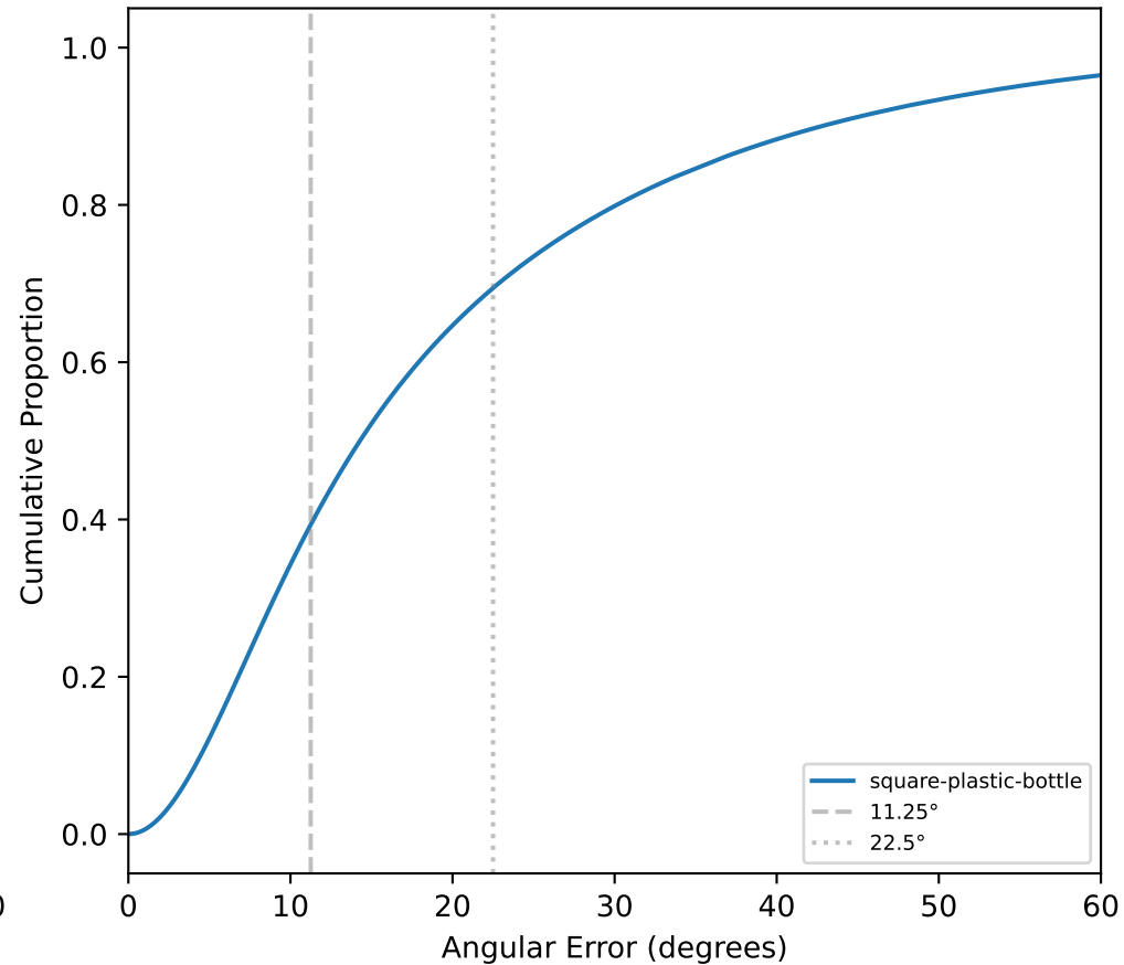
Threshold-Accuracy Curve
