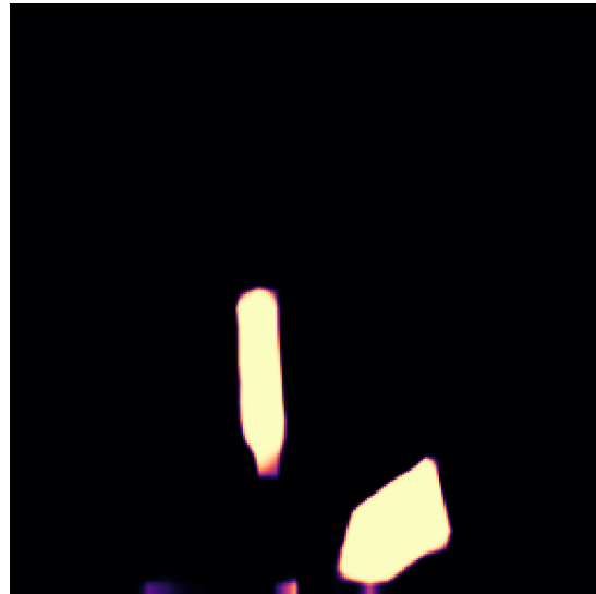
Predicted Logits
