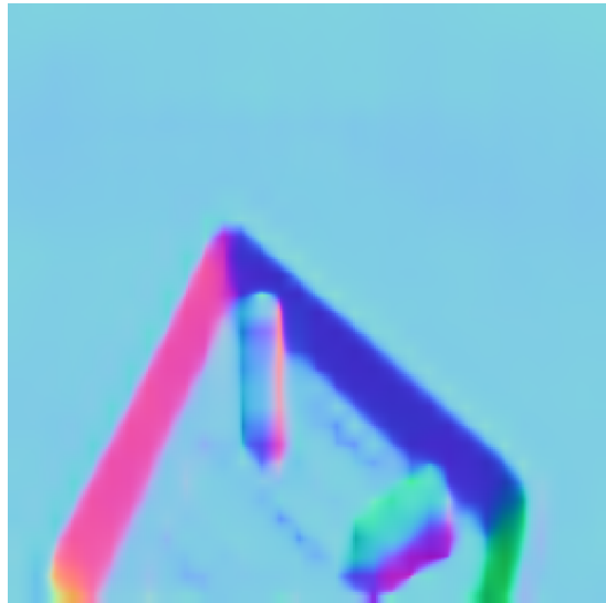
Predicted Normals
