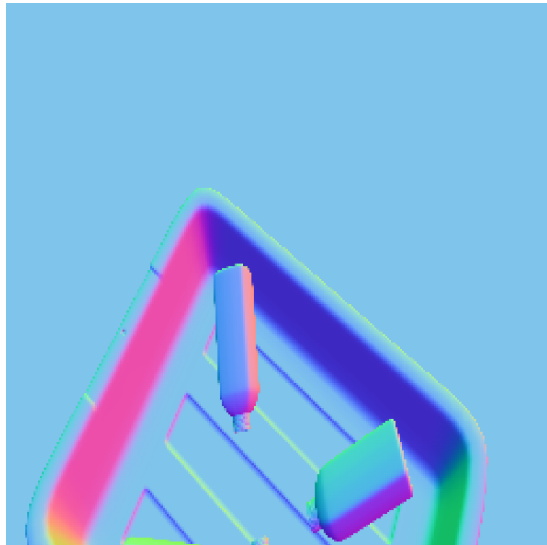
Ground-Truth Normals
