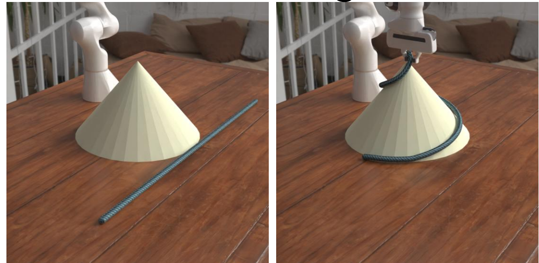
Slingshot
