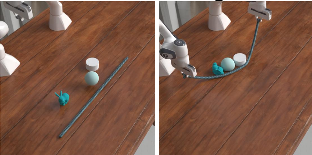
Unknotting
