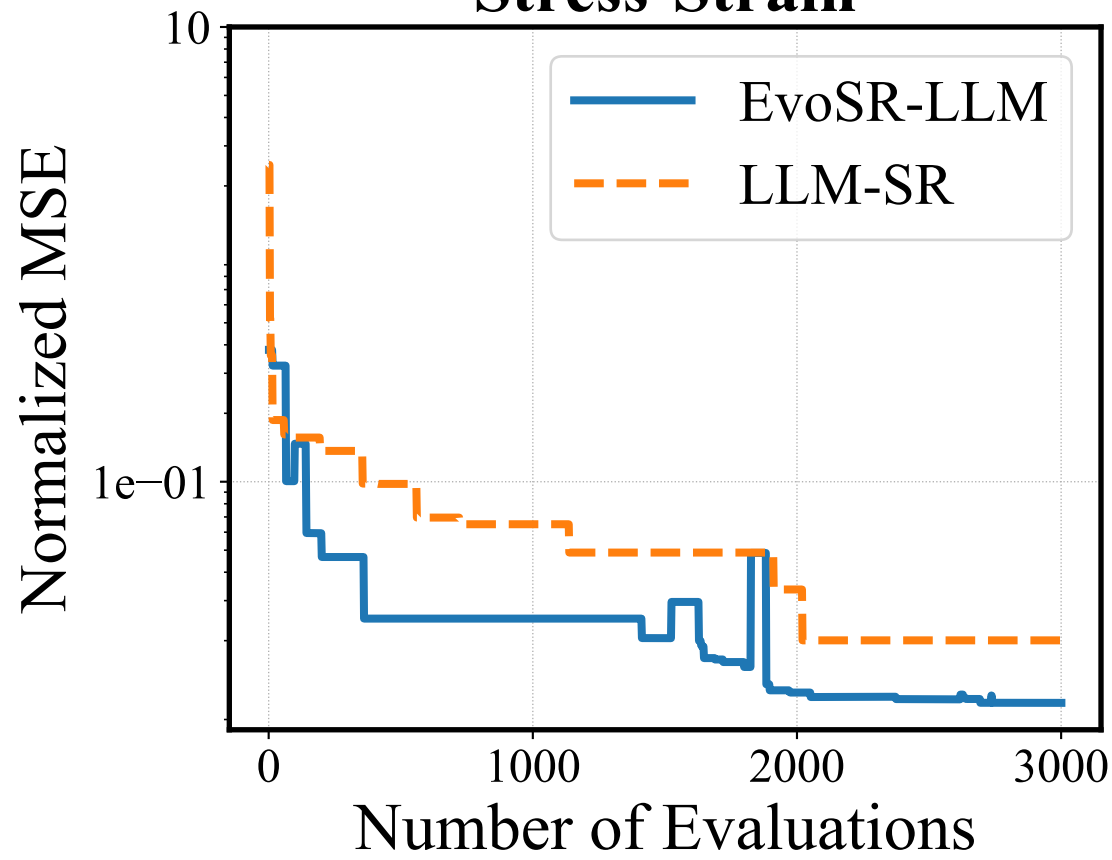
Stress-Strain
