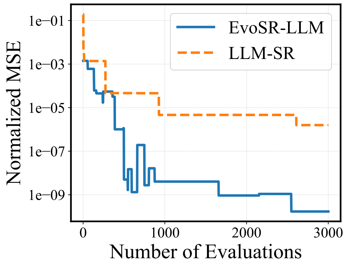
Oscillator 2
