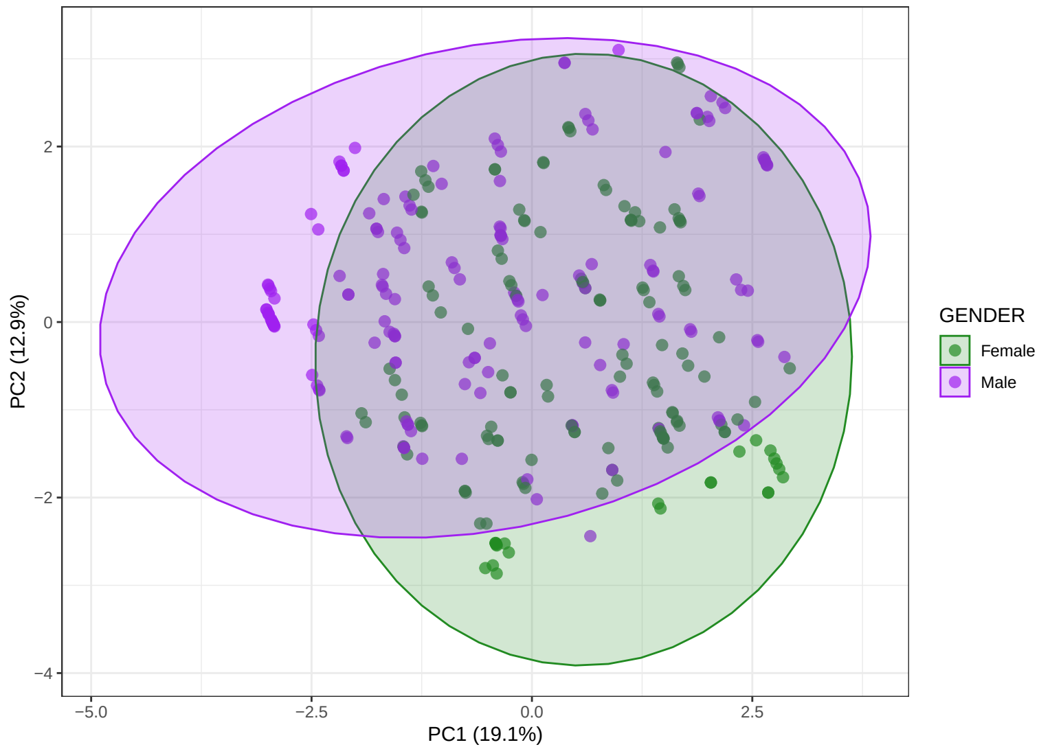
PCA Score Plot: PC1 vs PC2 by Gender
