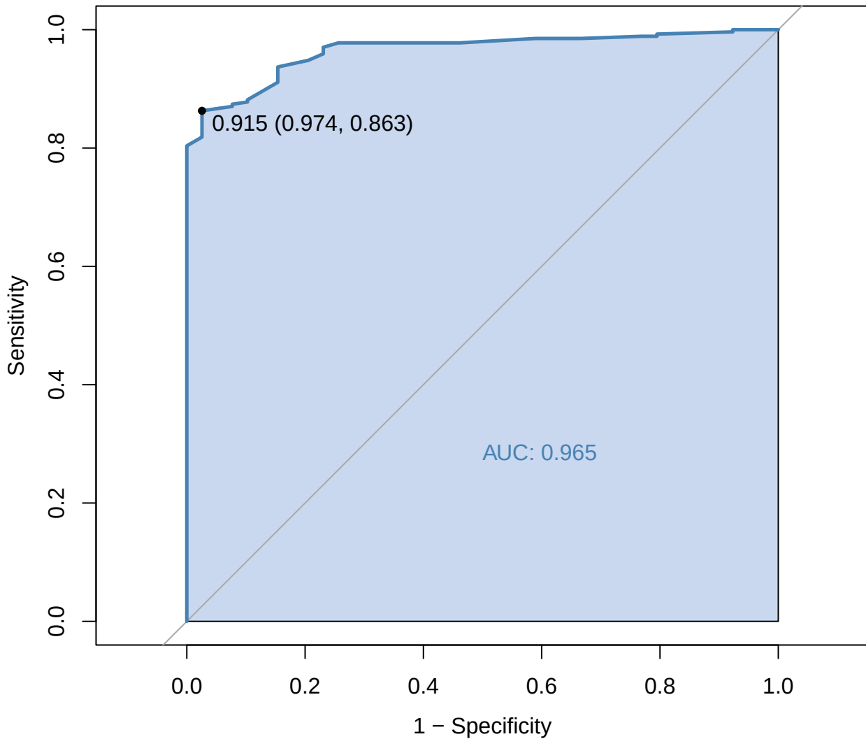
ROC Curve – Multivariate Logistic Model
