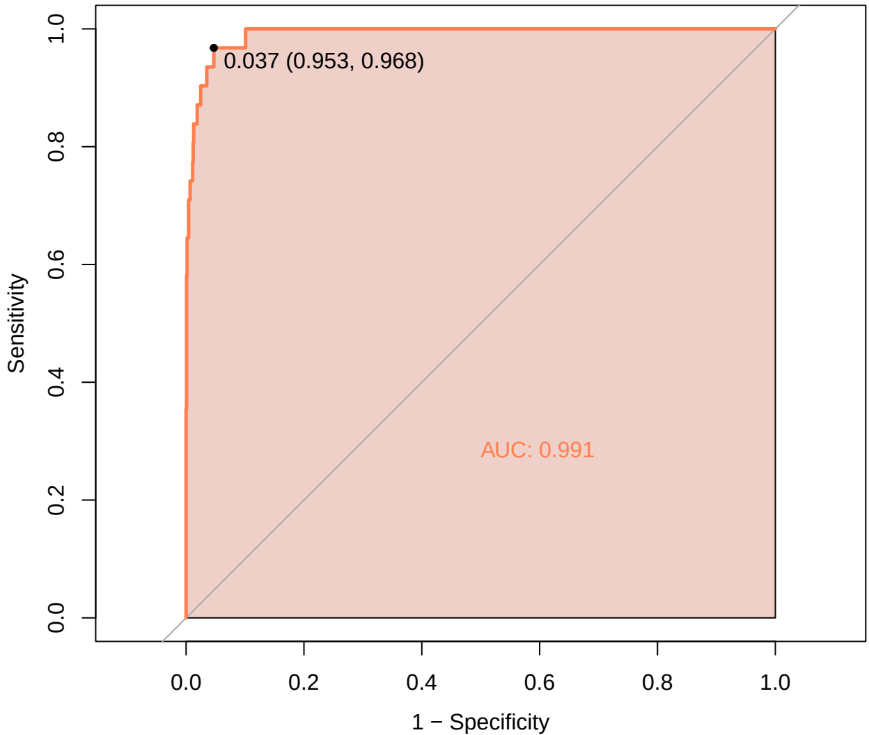
ROC Curve – Depression Prediction
