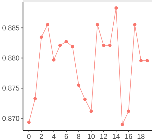
Balanced clusters
