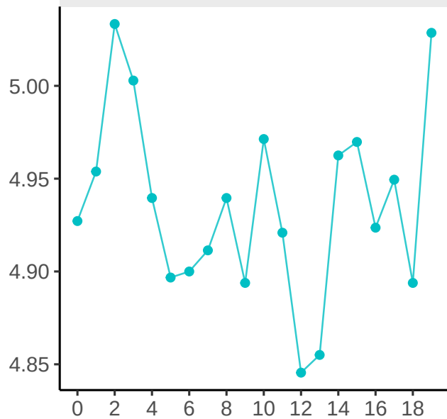
Imbalanced clusters
