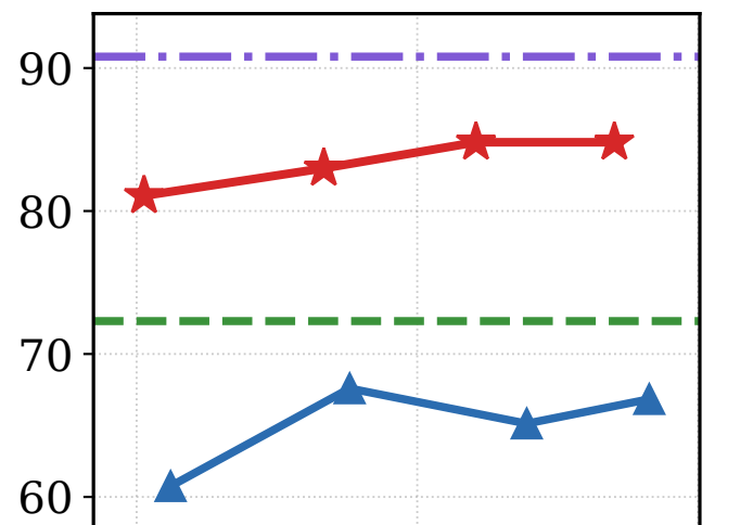
En-De
