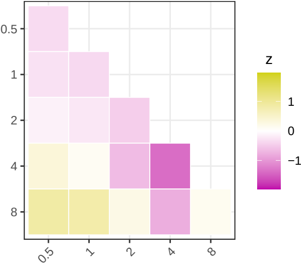
Standardised residual
