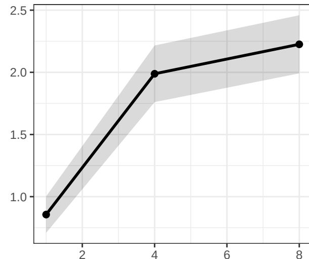
Standardised residual
