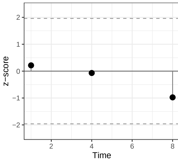
Standardised residual
