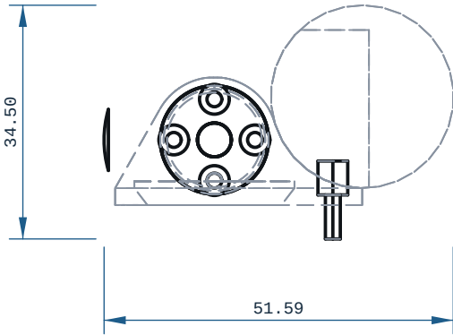
RIGHT VIEW -Y ? Z ?
