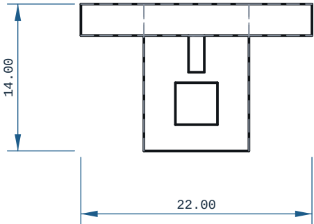
FRONT VIEW -X ? Z ?
