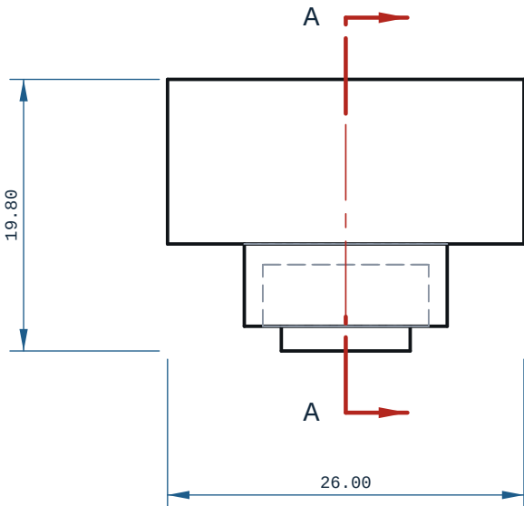
FRONT VIEW -X ? Z ?
