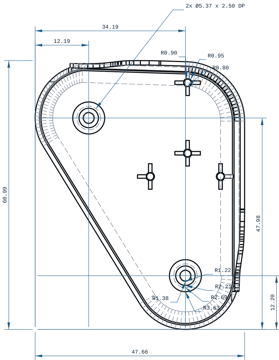
RIGHT VIEW
