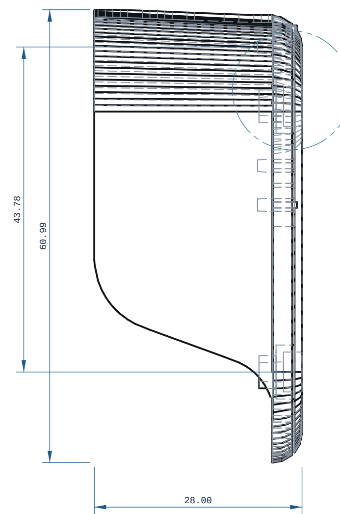
FRONT VIEW
