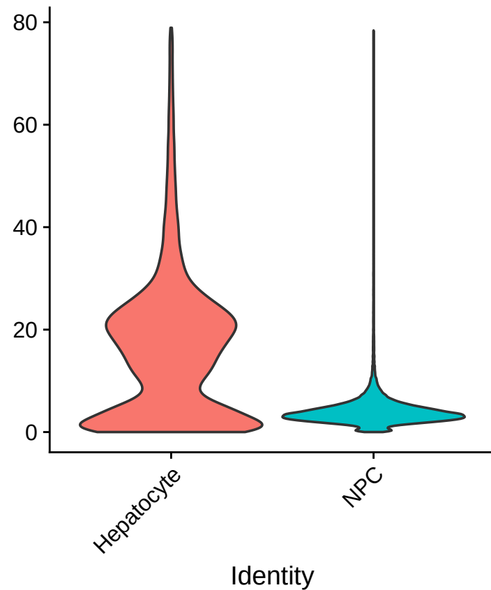
percent.mt
