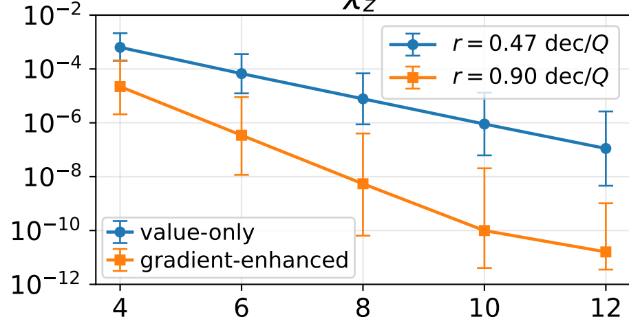
held-out error
