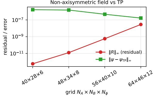
FIG. 8. Non-axisymmetric data validated against TwoPunctures. For a misaligned-spin configuration ( S^A = (0.3, 0, 0.2) , b = 1.5 , P = 0.5 ), the conformal factor converges spectrally toward the TwoPunctures solution ( \|\psi - \psi_{TP}\|_\infty , squares) and continues to decrease at the highest resolution considered. The certified Newton–Krylov residual \|R\|_\infty (circles) is near machine precision at the production resolution. Its slow increase at higher meridional resolution results from roundoff amplification in unpopulated high- m modes (Sec. VII) rather than from a loss of convergence, as the field difference continues to decrease. Here \|R\|_\infty is the row-equilibrated residual of Sec. III B, evaluated at the returned iterate.
