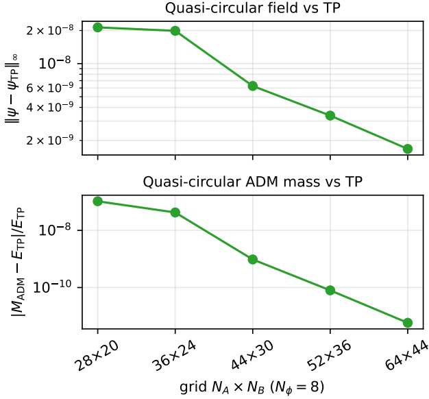
FIG. 9. Quasi-circular data validated against TwoPunctures. For a nonspinning, equal-mass quasi-circular configuration with b = 4 , (top) the conformal factor converges spectrally toward the TwoPunctures solution, reaching \|\psi - \psi_{TP}\|_\infty = 1.7 \times 10^{-9} and still decreasing at the highest resolution considered, while (bottom) the ADM mass converges approximately three orders of magnitude further. Both panels share the resolution axis.
