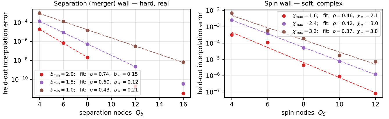
FIG. 2. The two analyticity walls: separation (hard, real) versus spin (soft, complex). Held-out interpolation error against the number of nodes along each axis, for a range of sampling intervals, with the geometric fit \varepsilon \approx A 10^{-\rho Q} overlaid (dashed). Each fit spans only the clean geometric window, so a dashed line stops short of the full node range wherever the error has already saturated on the float64 floor. Each legend entry gives, for its sampling range, the fitted rate \rho (decades/node) and the inferred nearest real singularity \theta_* . Left (merger wall, in the separation b ): the rate degrades as the interval is pushed toward coincidence while \theta_* stays pinned at b_* \approx 0 — a hard real singularity fixed at the merger. Right (spin wall, in \chi ): the rate degrades only mildly and \chi_* marches outward, remaining beyond the sampled range — the signature of a complex-conjugate pair off the real axis (Sec. VC). [TODO: caption rebuild — the figure is now THREE panels, separation | q | spin. The bold title (“The two analyticity walls...”) and the Left/Right pointers must become Left/Middle/Right, with a self-contained sentence for the mass-ratio panel (its character is unmeasured, so the panel title carries no claim yet). Every number in this figure also changes with the rebuild: the current curves are from the superseded narrow box b \in [1.5, 4] in the old bare-spin ( S_{Ay}, S_{By} ) parameterization, not the production box.]
