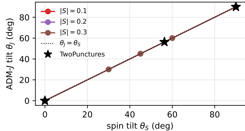
(a) ADM- J tracks the spin
