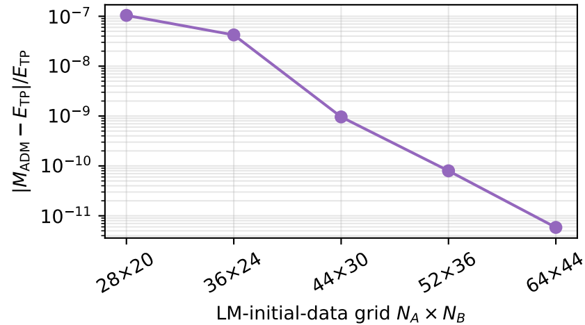
(c) quasi-circular ADM mass vs TP
