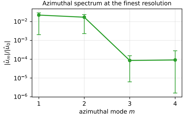
FIG. 9. Azimuthal structure of the quasi-circular data. Azimuthal Fourier spectrum |\hat{u}_m|/|\hat{u}_0| at the finest resolution: median with min-max whiskers over the same 100 configurations as Fig. 8, with m = 0 the normalization and not shown. The last point is that grid's Nyquist mode (dotted): \sin 4\phi vanishes identically on N_\phi equispaced nodes, so it carries only the \cos 4\phi component, one real degree of freedom against two for m = 1-3 , and is not comparable like-for-like with them.
