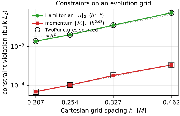
FIG. 10. Constraint violation of the initial data on a uniform Cartesian evolution grid. Bulk L_2 norms of the Hamiltonian and momentum constraints against the Cartesian grid spacing h , for the axisymmetric configuration of App. A 1 (equal bare masses, half-separation b = 3 , axial momentum P = 0.5 ), on the four grids N^3 with N = 40, 56, 72, 88 across a box of half-width 9M with the punctures excluded to radius 1.5M . Both norms are measured by the generic finite-difference constraint monitor described in the text, which makes no use of conformal flatness, and both fall at its second order (measured 2.14 and 2.02; dotted, \propto h^2 ). Black open markers repeat the measurement with the conformal factor supplied by TwoPunctures on the same grids; the two agree to better than 10^{-6} relative at every rung, so what is plotted is the truncation error of the Cartesian discretization rather than a property of either initial-data solution.
