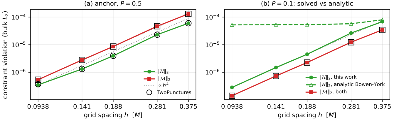
FIG. 10. Constraint violation of the initial data, measured by an independent evolution code. Volume-normalized bulk L_2 norms of the Hamiltonian and momentum constraints at t = 0 , computed by GRTeclyn [37] with its own fourth-order stencils from the evolution variables of the CCZ4 system, against the grid spacing h on a uniform ladder h = 0.375\text{--}0.094 M ( N^3 with N = 48, 64, 96, 128, 192 ) across a box of half-width 9 M , with the punctures excluded to radius 1.5 M . (a) The axisymmetric configuration of App. A 1 (equal bare masses, half-separation b = 3 , axial momentum P = 0.5 ). Both norms fall at the operator's fourth order, the measured local orders being 3.32, 4.35, 3.82, 3.27 for \|\mathcal{H}\|_2 and 3.57, 4.17, 3.91, 4.06 for \|\mathcal{M}\|_2 (dotted, \propto h^4 ). Black open markers repeat the measurement with the conformal factor supplied by TwoPunctures, passed through the identical initial-data class, interpolation, stencils and grid, so that the initial data is the only difference: the two agree to 6 \times 10^{-6} relative at the coarsest rung and to 6 \times 10^{-2} at the finest, where the violation is itself 3.5 \times 10^{-7} . (b) The same configuration at P = 0.1 , the largest momentum for which GRTeclyn's own analytic Bowen-York initial data is defined (it requires |P| < 0.3 m , so it cannot represent the P = 0.5 anchor at all). Our Hamiltonian violation continues to fall at fourth order; the analytic one stops falling at 5.2 \times 10^{-5} (local orders 0.19, 0.01, 0.03) and ends a factor 184 higher, because that data satisfies the Hamiltonian constraint only to O(P^2) . The momentum norms coincide to three digits, as they must: the Bowen-York extrinsic curvature is analytically transverse in both, so the momentum constraint holds for any conformal factor and both curves are pure truncation error. Panel (b) therefore isolates the Hamiltonian sector, which is the sector in which the two data sets differ.
