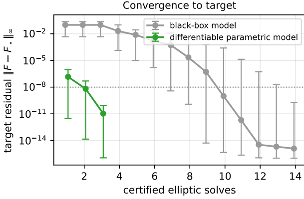
FIG. 6. Certified parameter targeting. Reaching a physical target ( M_{\text{ADM}}, J ) by adjusting (b, q) , over 100 random known-answer targets, measured in certified elliptic solves. Each method is drawn as the across-target median residual at each solve count, with min-max whiskers; every target is carried to a common solve count, so each point is the full set of 100. Each curve ends where its last target reaches the control tolerance (dotted): three certified solves for the differentiable parametric model, with a median of two, against fourteen for the black-box loop, with a median of ten.
