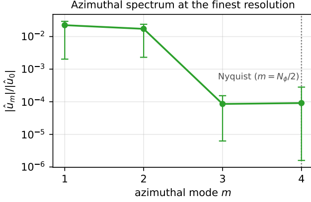
FIG. 9. Azimuthal structure of the quasi-circular data. The azimuthal Fourier spectrum |\hat{u}_m|/|\hat{u}_0| at the finest resolution, which shows where the non-axisymmetric content of these data sits. Median with min-max whiskers over the same 100 configurations as Fig. 8; m = 0 is the normalization and is not shown. The expansion of Eq. (15) carries |m| \leq N_\phi/2 , so the production grid, at N_\phi = 8 , reaches m = 4 and every mode it represents is plotted. The last point is that grid’s Nyquist mode (dotted): \sin 4\phi vanishes identically on N_\phi equispaced nodes, so it carries only the \cos 4\phi component, one real degree of freedom against two for m = 1 –3, and is not comparable like-for-like with them. Content above m = 4 would fold into the plotted modes rather than appear beyond them, so the panel bounds the high- m amplitudes rather than resolving them; that N_\phi = 8 suffices follows from refinement, reported in the text.
