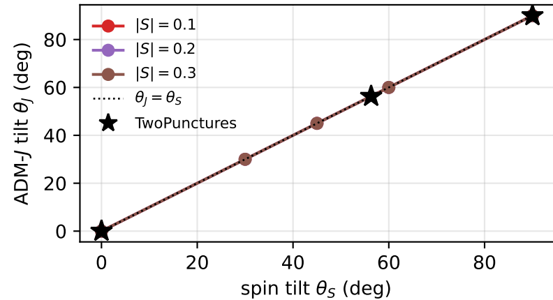
(a) ADM- j tracks the spin
